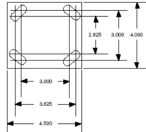
HOLES FOR 0.3125 BOLTS
