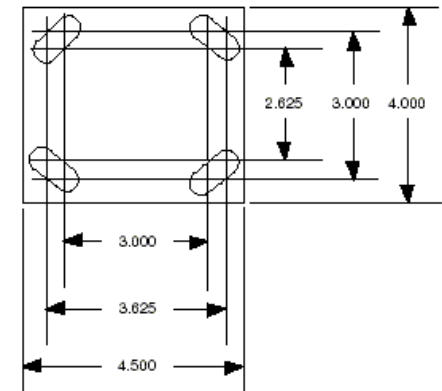
HOLES FOR 0.3125 BOLTS
